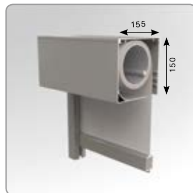
Doorsnede Fixscreen® 150 EVO (F)
